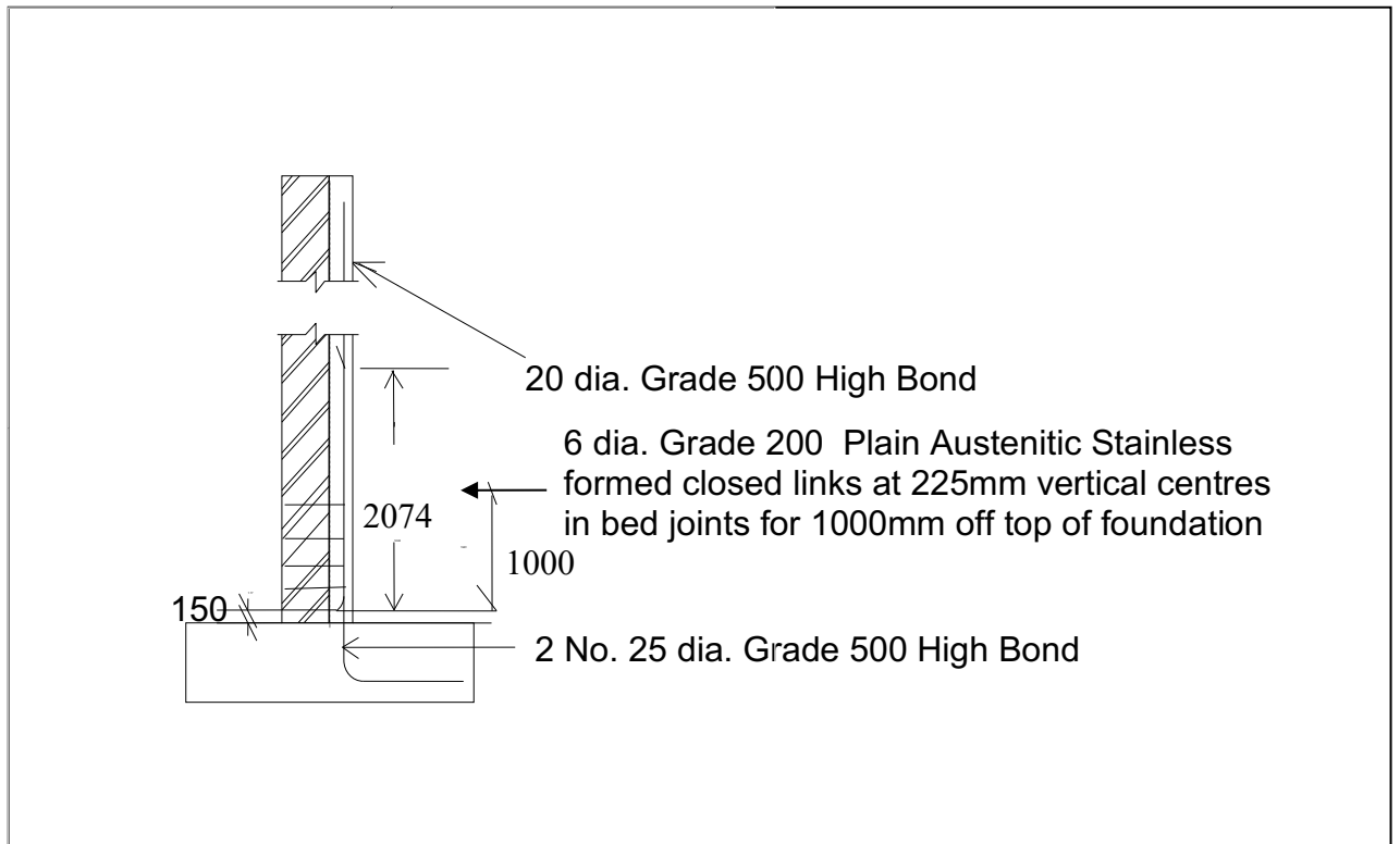
Figure 2: Arrangement of reinforcing steel
